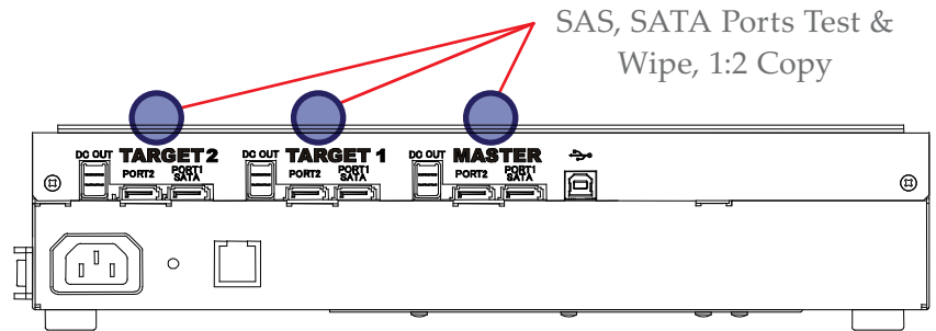
Back view
